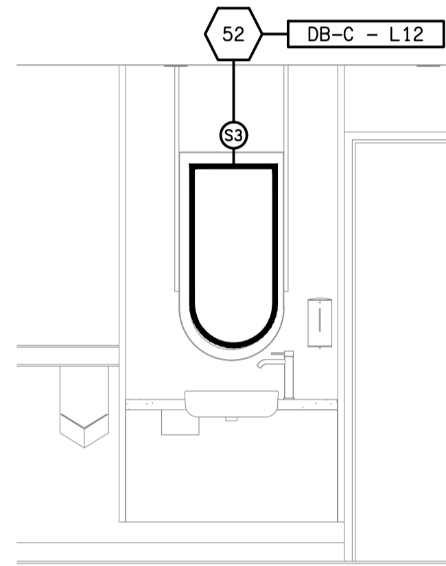
DETAIL D FEMALE MIRROR ELEVATION SCALE 1:25
